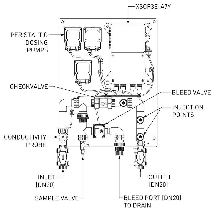
FRONT (1:6)
