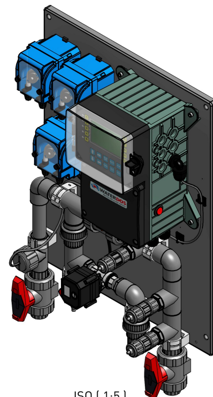
ISO (1:5)
