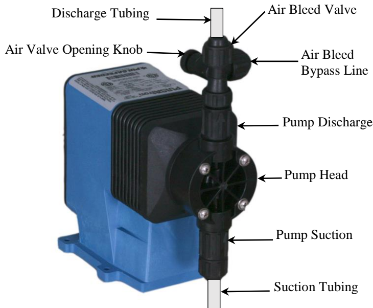
Figure 9 Air Bleed Valve Configuration
