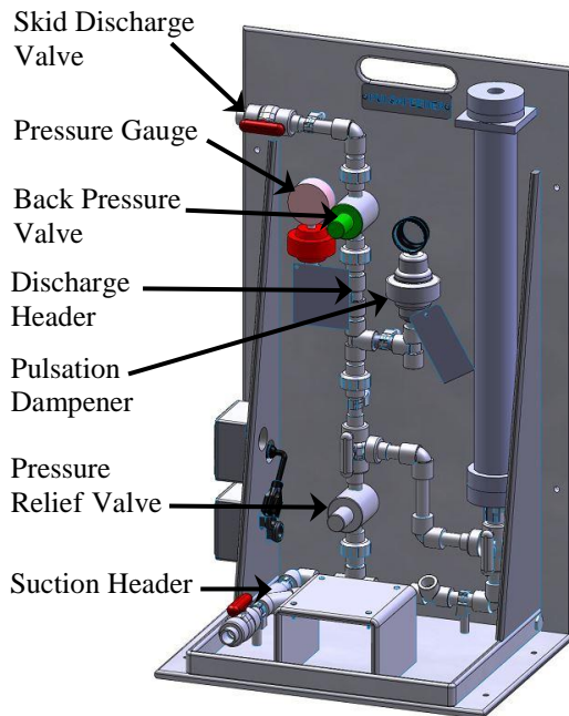
Figure 12 Skid Component Locations
