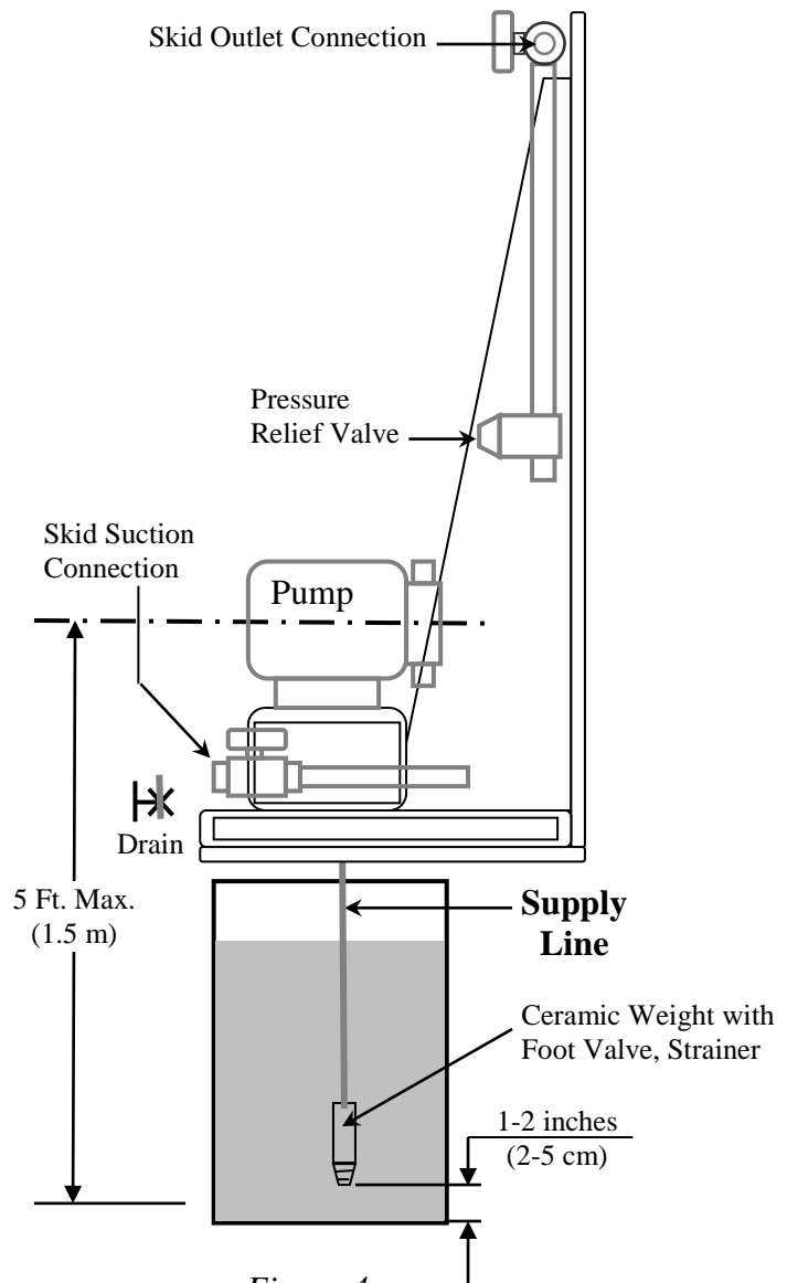
Figure 4 Suction Lift
