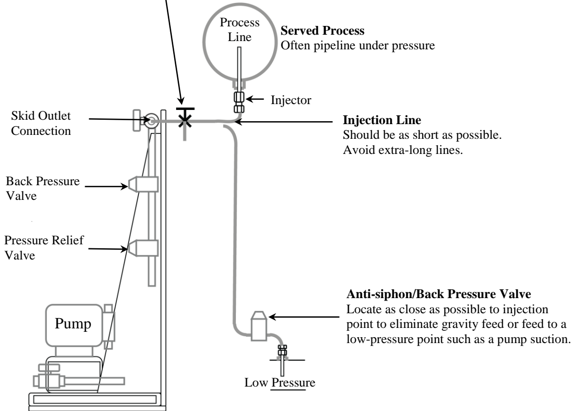
Figure 5 Process Piping Considerations
